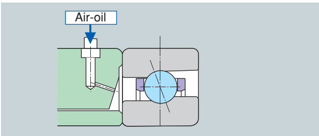
Fig. 8.7 Standard nozzle
