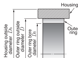
Fig. 6.17 Fit between outer ring and housing
