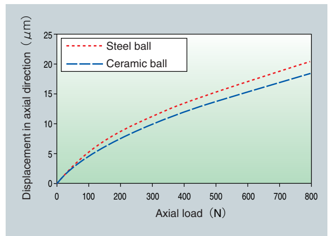
Fig. 9.20 Displacement in axial direction
