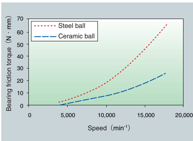
Fig. 9.19 Frictional torque
