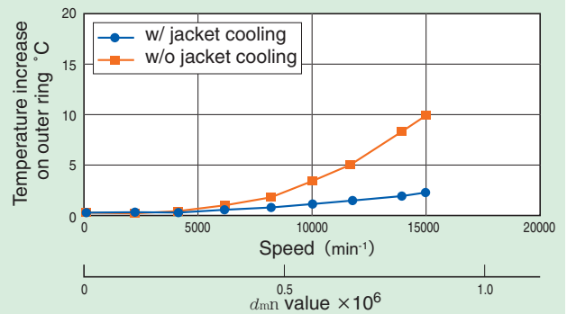
Fig. 9.22 High-speed test with grease lubrication
