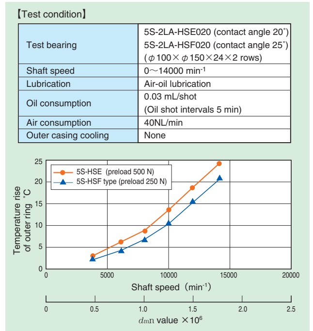
Fig. 9.28 Comparison of temperature rise
