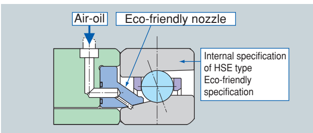
Fig. 8.8 Eco-friendly type nozzle
