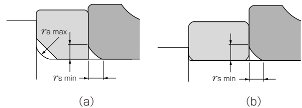
Fig. 2.16 Bearing mounting with spacer
