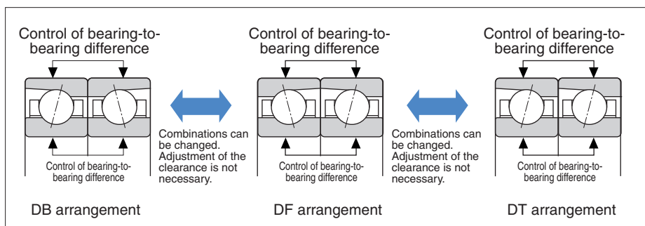
Fig. 9.14 Universal matching
