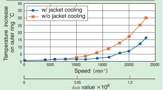
Fig. 9.23 High-speed test with air-oil lubrication
