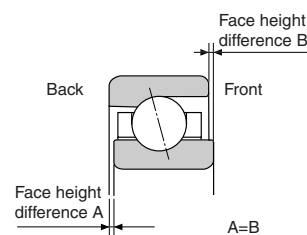
Fig. 9.13 Flush grinding
