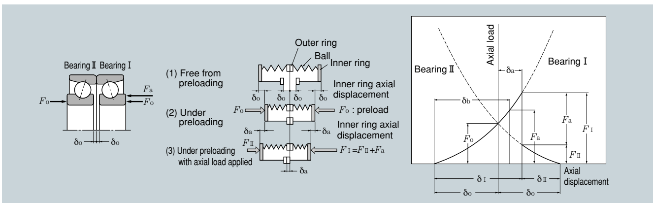
Fig. 2.11 Preload graph
