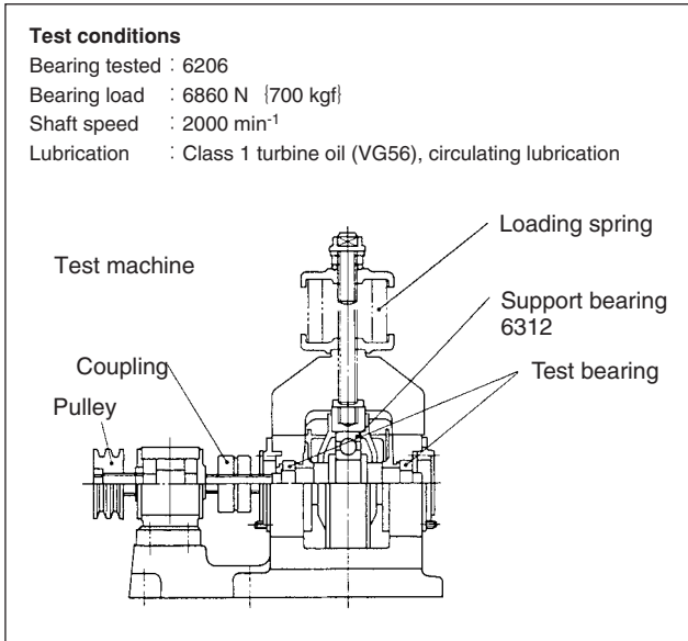
Fig. 9.17 Radial load-type bearing life test machine
